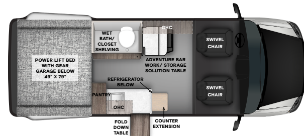
19 SCV - ADVENTURE BAR
