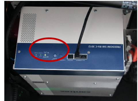
Figure 10-11: Converter/Inverter
