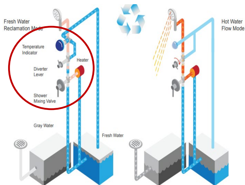
Figure 14-7: Shower Miser
