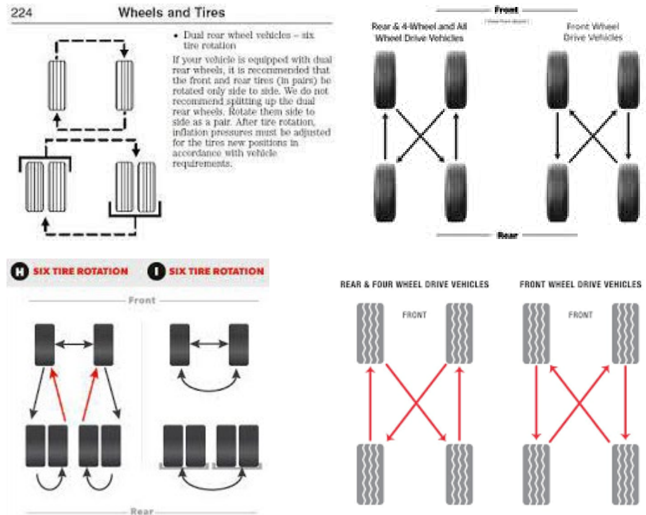
Figure 17-2: Vehicle Tire Rotation
