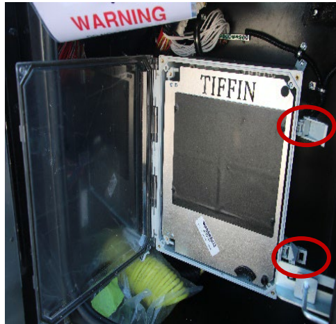
Step 1: Pull latches to open M1 Spyder Enclosure Door.
