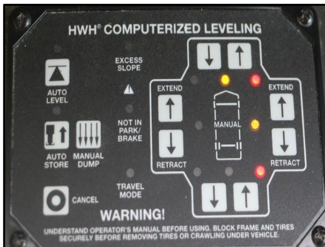
Figure 16-7: Leveling System Control Panel
