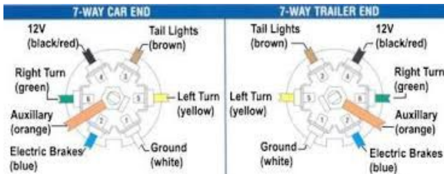
Figure 10-21 Connector Diagram
