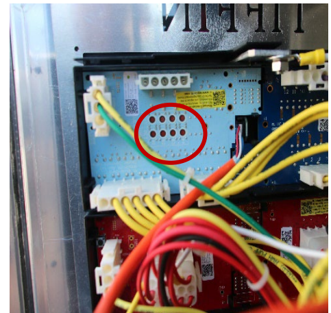
Step 5: Insert a round dowel in the control buttons to operate the Slide-Out Room.
