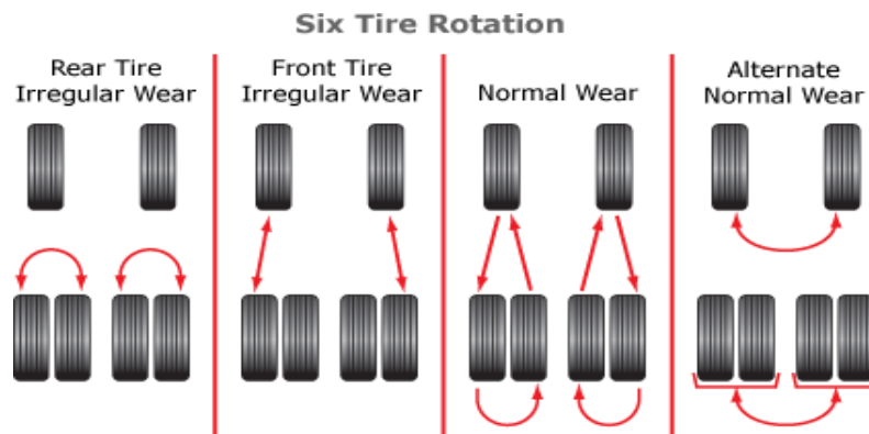
Figure 17-2: Vehicle Tire Rotation
