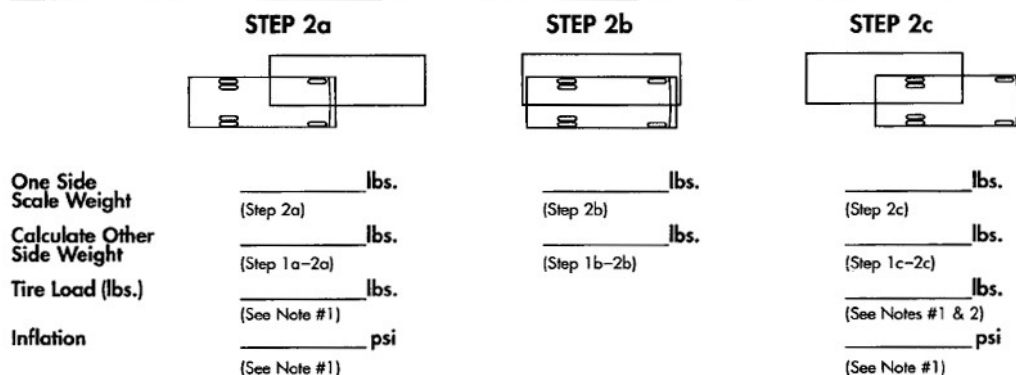
Figure 17-5: Motorhome Weighing Procedures
