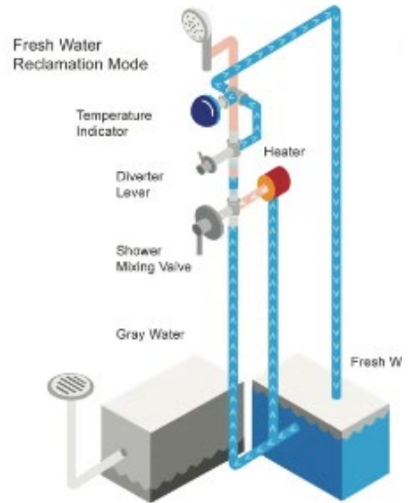
Figure 9-5: ShowerMiser
