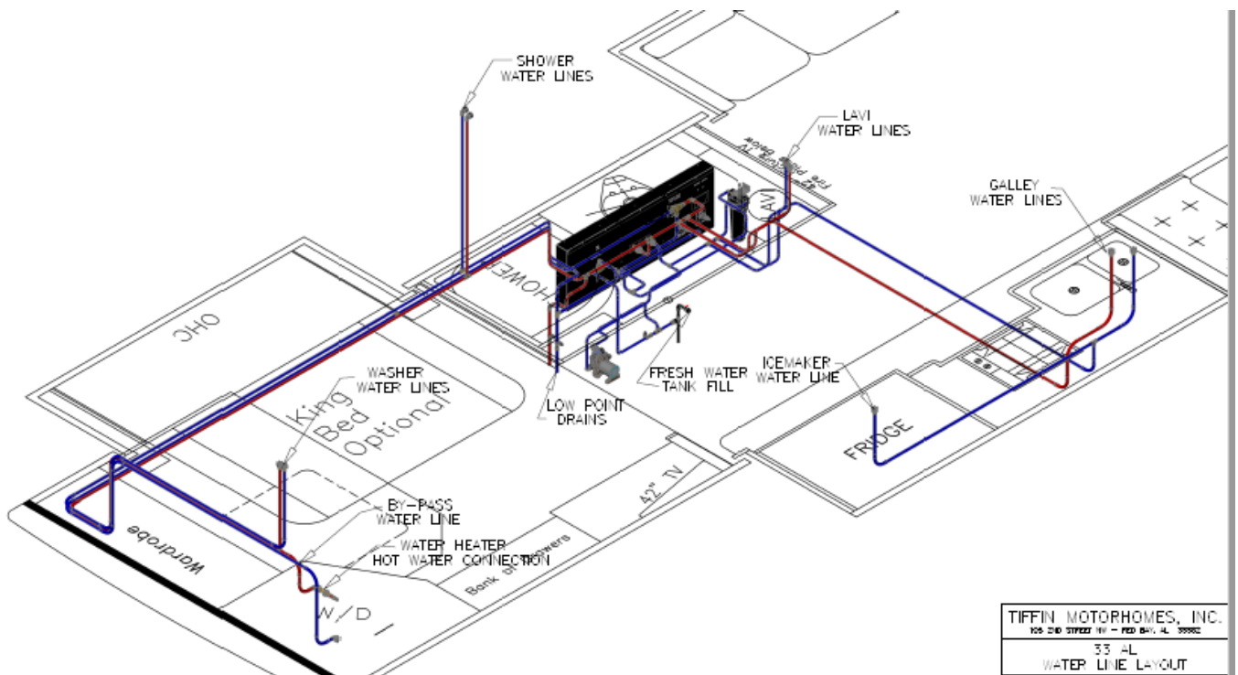
Water Line Layout
