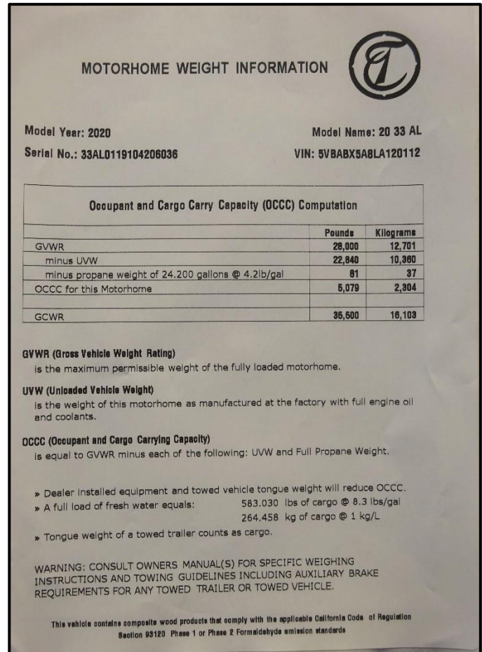
Figure 0-4: Sample Motorhome Weight Label (found in the bedroom closet)
