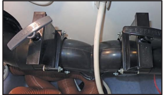
Figure 0-11: Sanitation Coupling
