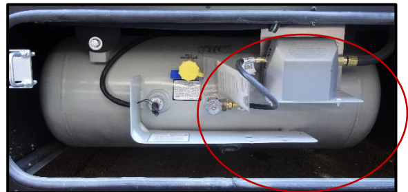
Figure 0-2: LP Gas Regulator
