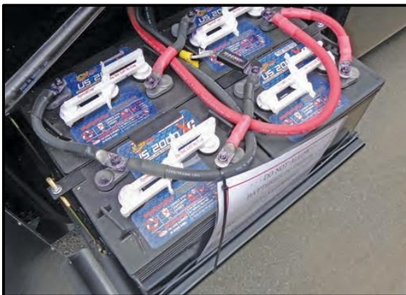
Figure 0-14: House Batteries
