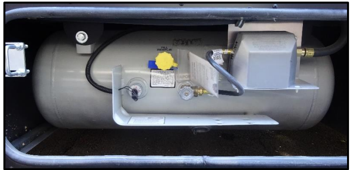
Figure 0-3: LP Tank and Regulator
