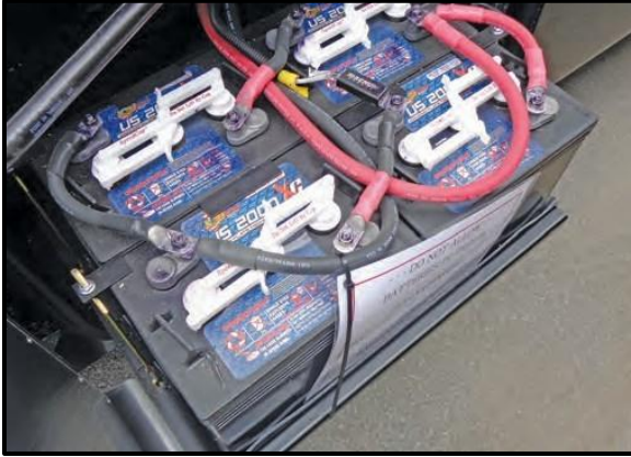
Figure 0-14: House Batteries
