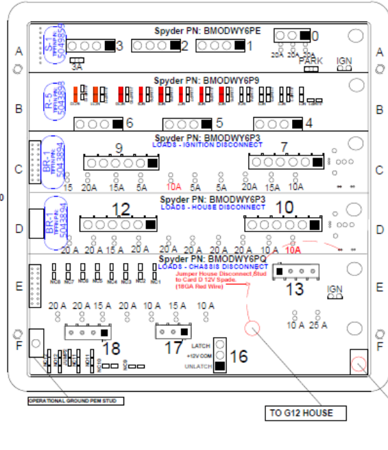
G6A CONTROL PANEL LAYOUT Tiffin PN: 5083668 Spyder PN: BENC254CL Bay - CHASSIS Rev 0VA PINOUT DIAGRAM - 04.01.2019 Back View
