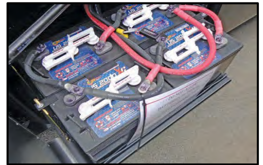
Figure 9-16: House Batteries
