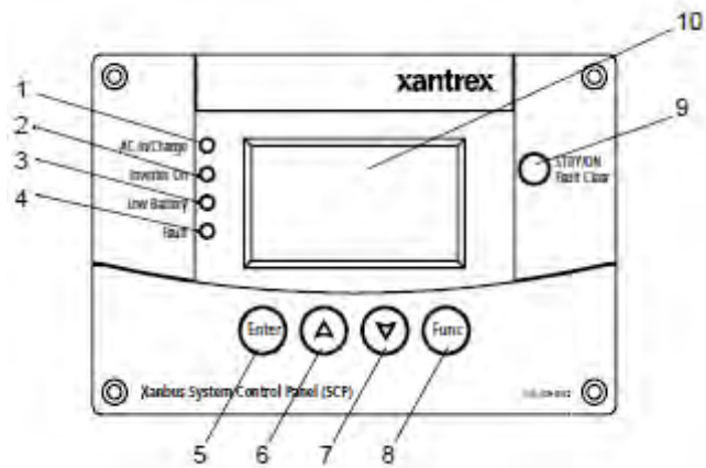
Figure 9-9: System Control Panel
