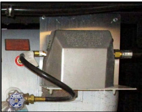
Figure 4-2: LP Gas Regulator
