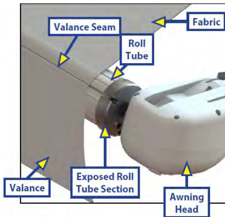
Figure 14-5: Extended Awning
