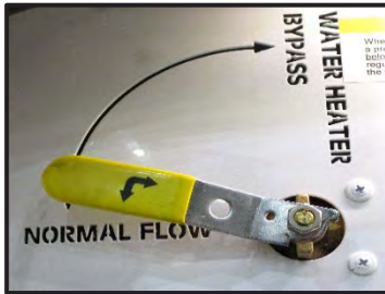
Figure 13-10: Water Heater Bypass System
