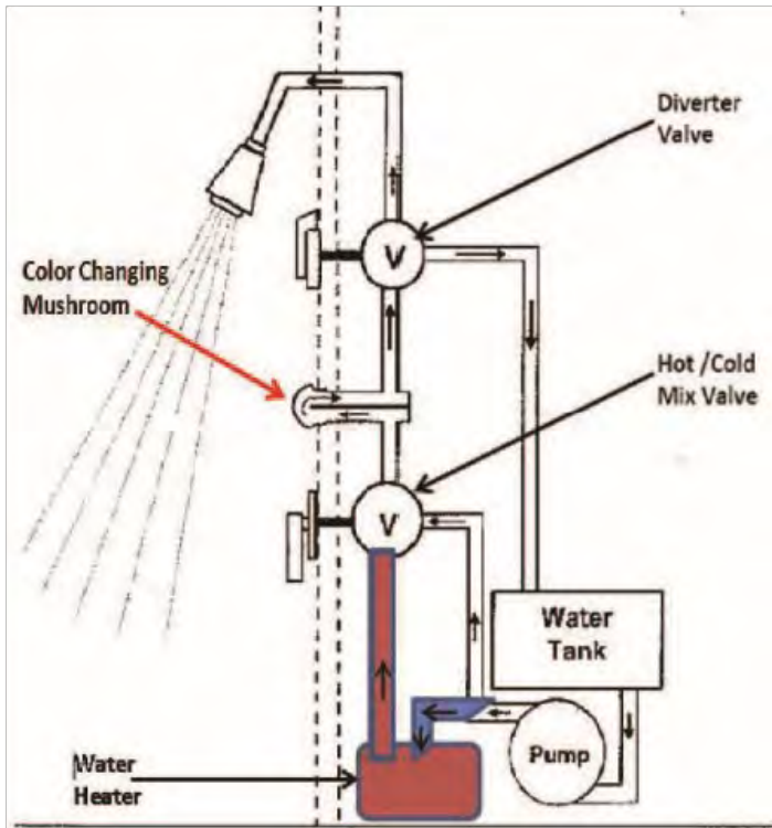
Figure 13-5: ShowerMiser™ Diagram.
