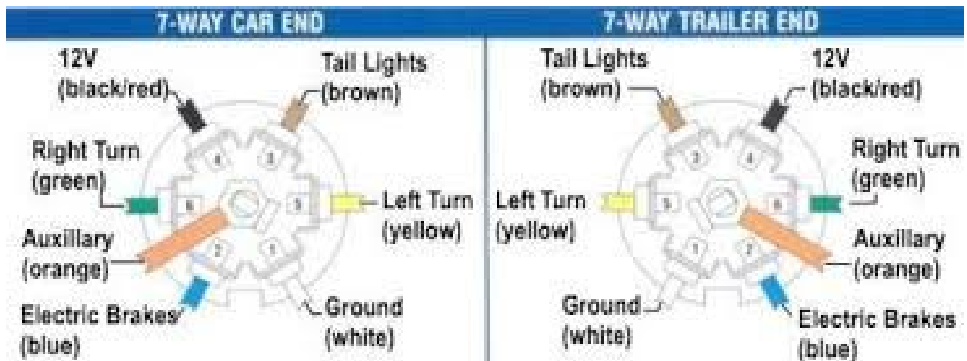
Figure 9-21 Connector Diagram
