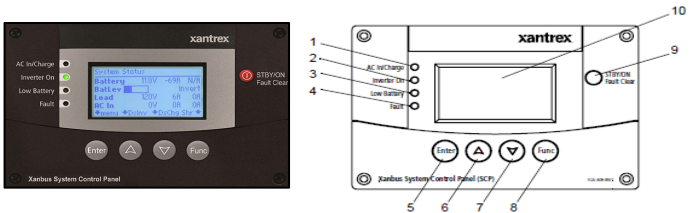
Figure 9-9: System Control Panel
