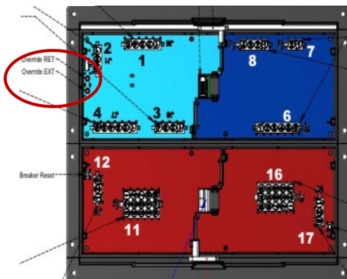
Figure 10-5: M1 Slide-Out Room Control Override behind the M1 Circuit Panel.
