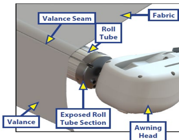
Figure 14-5: Extended Awning
