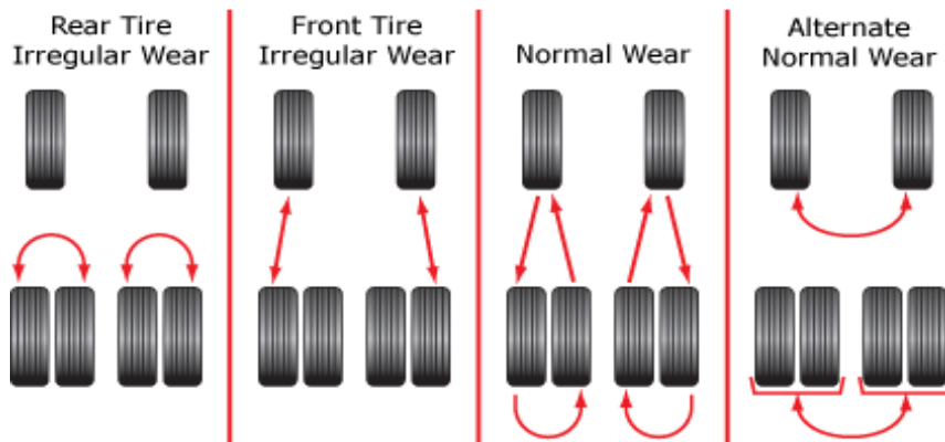
Figure 16-2: Tire Rotation
