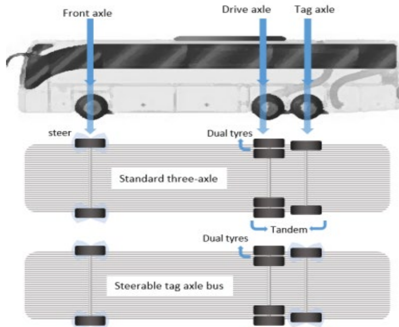
Figure 16-3: Vehicle Tire Information
