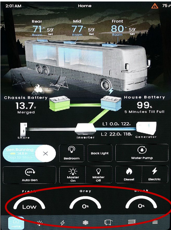
Figure 13-1: Tank-Level Monitor
