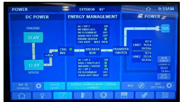
Figure 8-12: Control Panel for the Inverter/Charger
