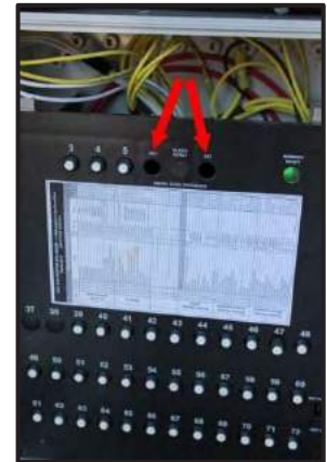
Figure 9-4: Location of Slide-Out Room Control Override
