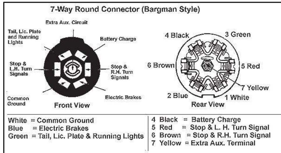
Figure 8-19: Seven-Pin Connector
