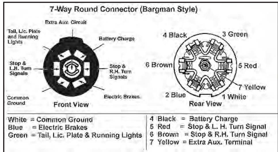
Figure 8-18: Seven-Pin Connector
