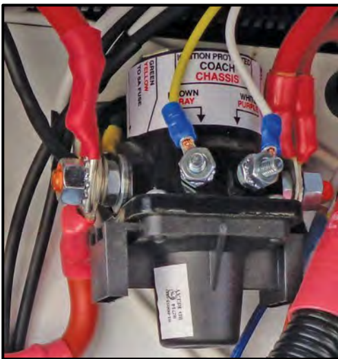
Figure 8-7: 12 VDC Disconnect Switch
