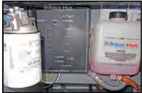
Figure 12-15: Aqua-Hot Surge Tank
