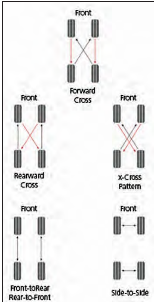
Figure 15-2: Tire Rotation
