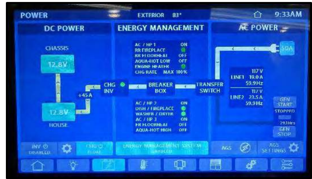
Figure 8-8: Multiplex System
