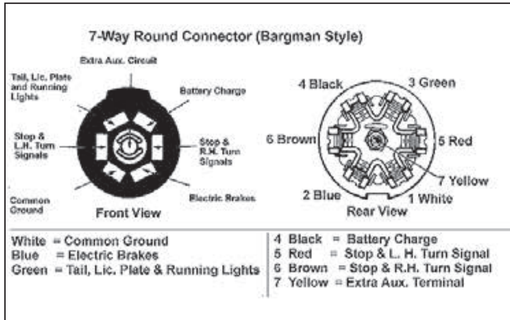
Figure 8-18: Seven-Pin towing connector
