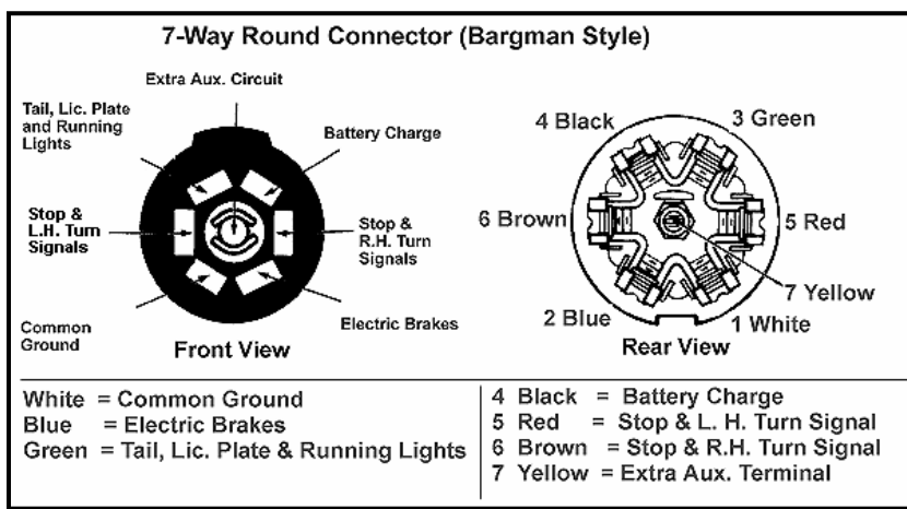
Figure 7-19. Bargman 7-Way Round Towing Connector
