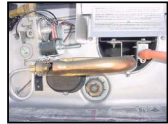
Figure 4-18. Water Heater Drain
