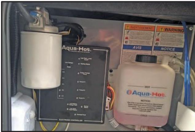
Figure 15-17: Surge Tank
