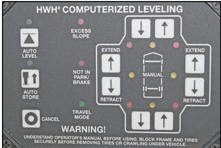
Figure 17-5: Leveling System Control Panel
