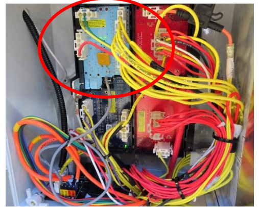
Figure 11-4: Location of Slide-Out Room Control Override behind the front panel.
