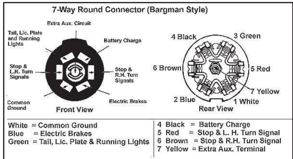
Figure 10-17: Seven-Pin Connector
