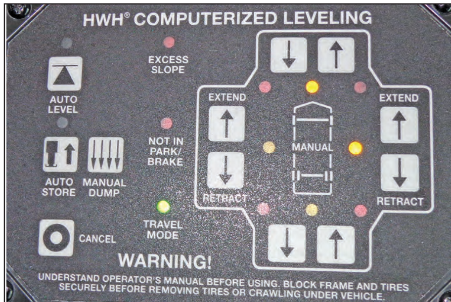
Figure 16-5: Leveling system control panel
