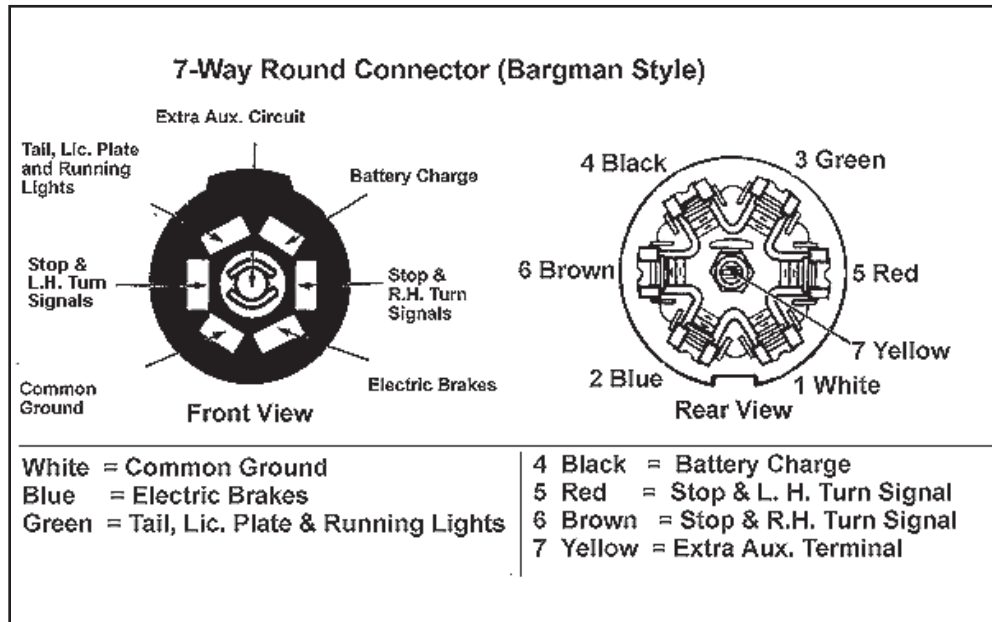
Figure 10-18: Seven-pin towing connector
