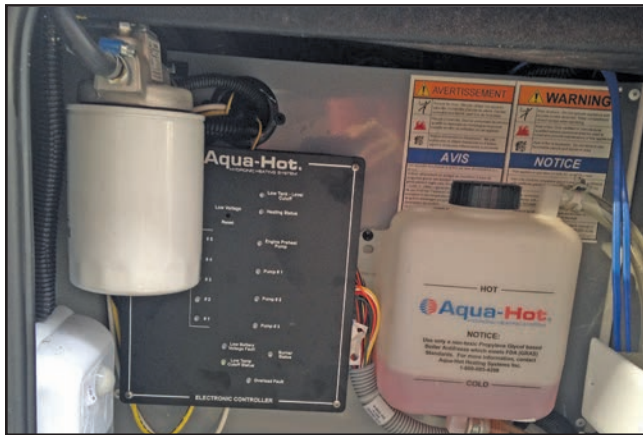
Figure 13-13: Surge tank
