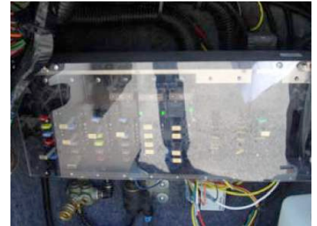
Figure 7-2. Fuse Panels
