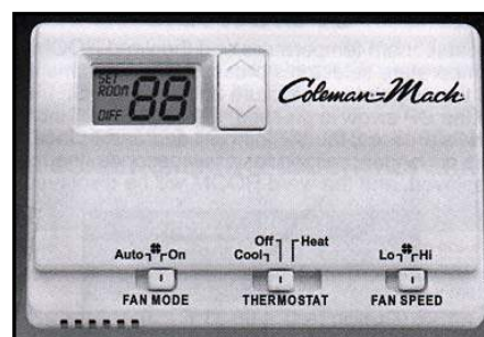
Figure 3-3. Thermostat
