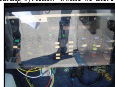
Figure 7-15. Fuse Blocks in exterior compartment on driver's side
