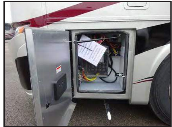
Figure 9-10: Circuit Breakers
