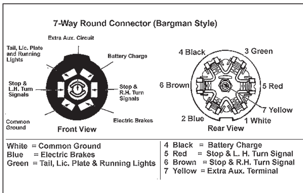
Figure 9-11: Seven-Pin towing connector
