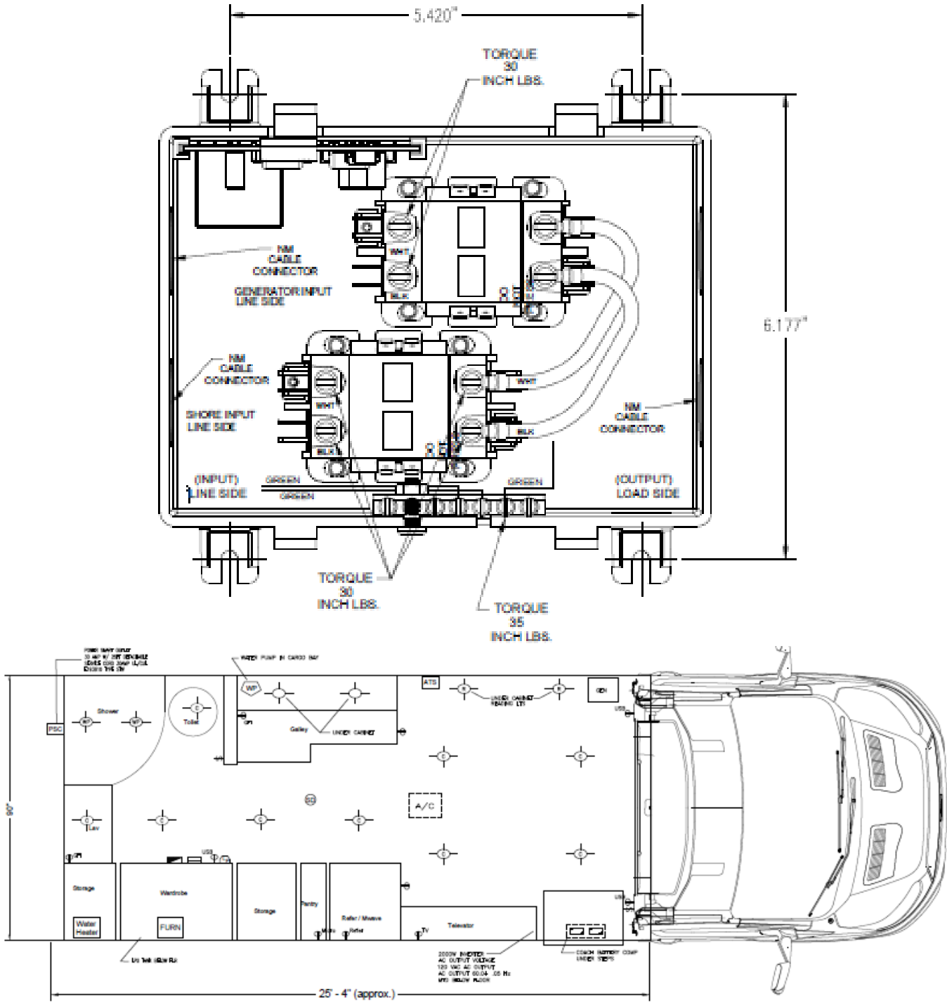
Electrical Floor Plan Layout Not To Scale
