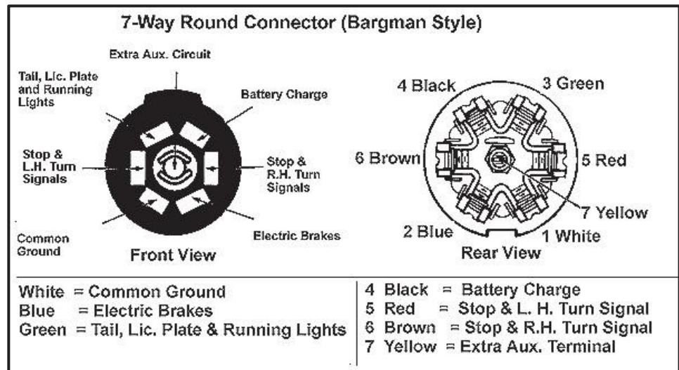
Figure 9-15: Seven-Pin Connector
