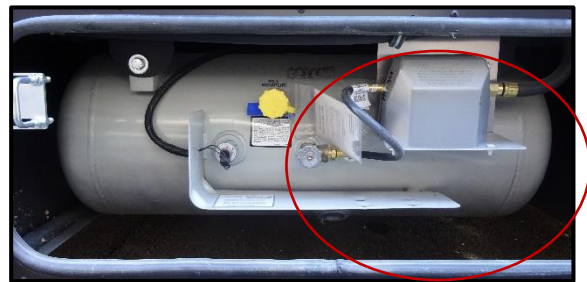
Figure 4-2: LP Gas Regulator
