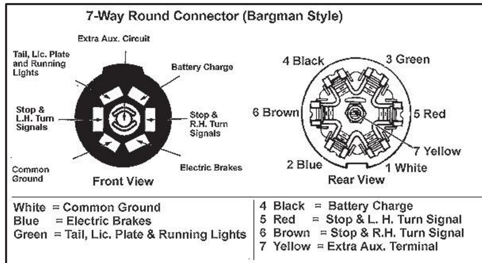
Figure 9-19: Seven-Pin Connector
