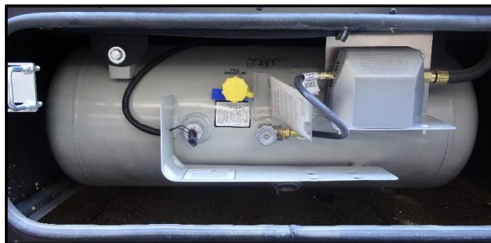
Figure 2-3: LP Tank and Regulator
