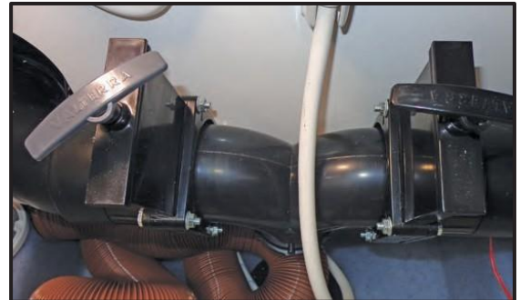
Figure 13-11: Sanitation Coupling
