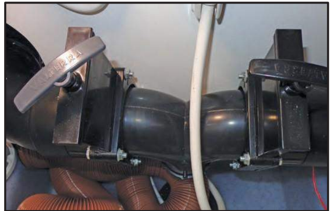
Figure 13-11: Sanitation Coupling
