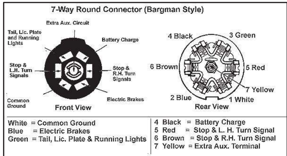
Figure 9-18: Seven-Pin Connector
