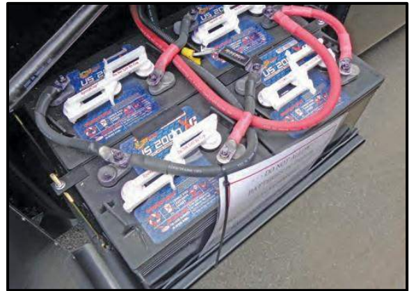
Figure 9-13: House Batteries
