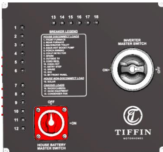
Figure 9-14: House Battery Disconnect Panel
