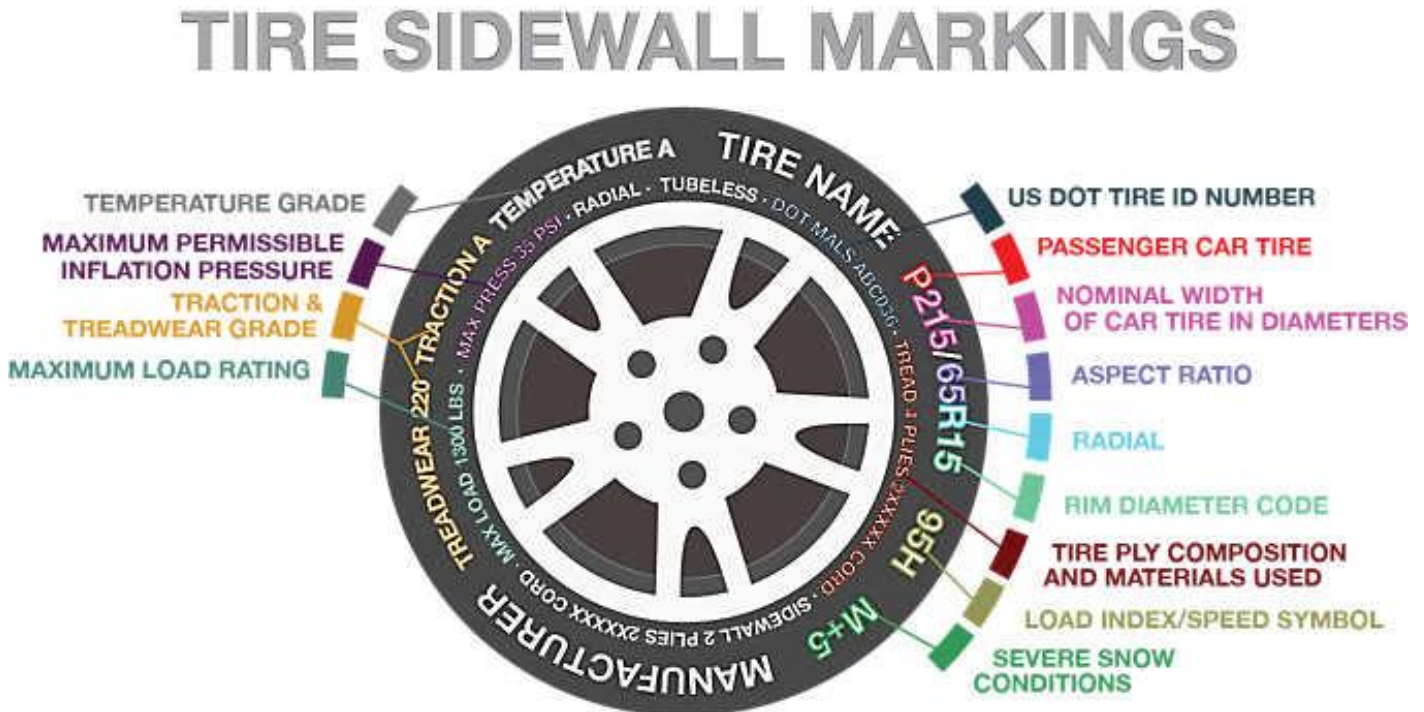
Figure 16-3: Vehicle Tire Information
