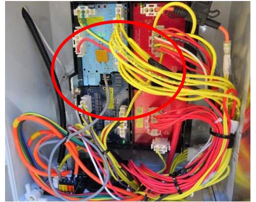
Figure 10-4: Location of Slide-Out Room Control Override
