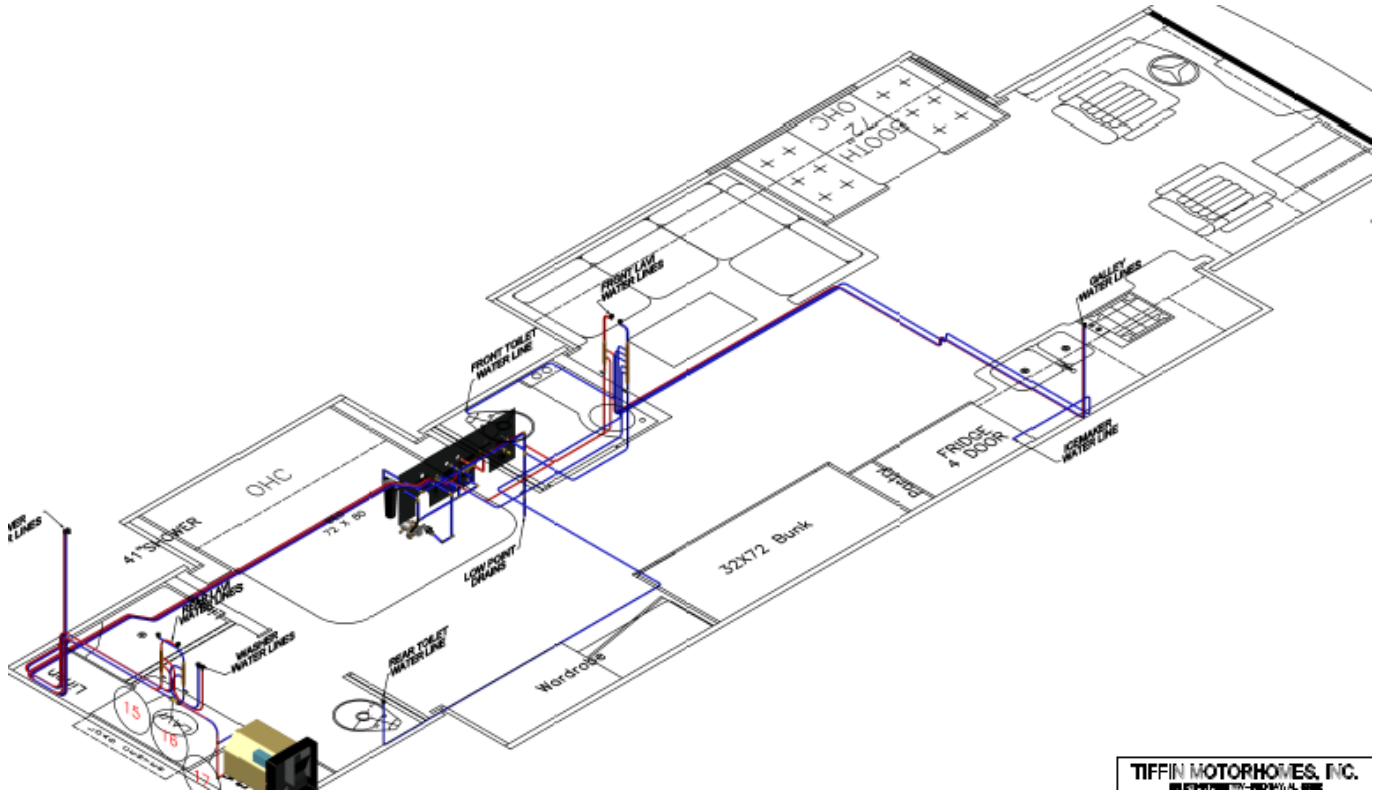
37BA Water Line Layout
