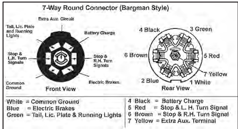
Figure 9-19: Seven-Pin Connector
