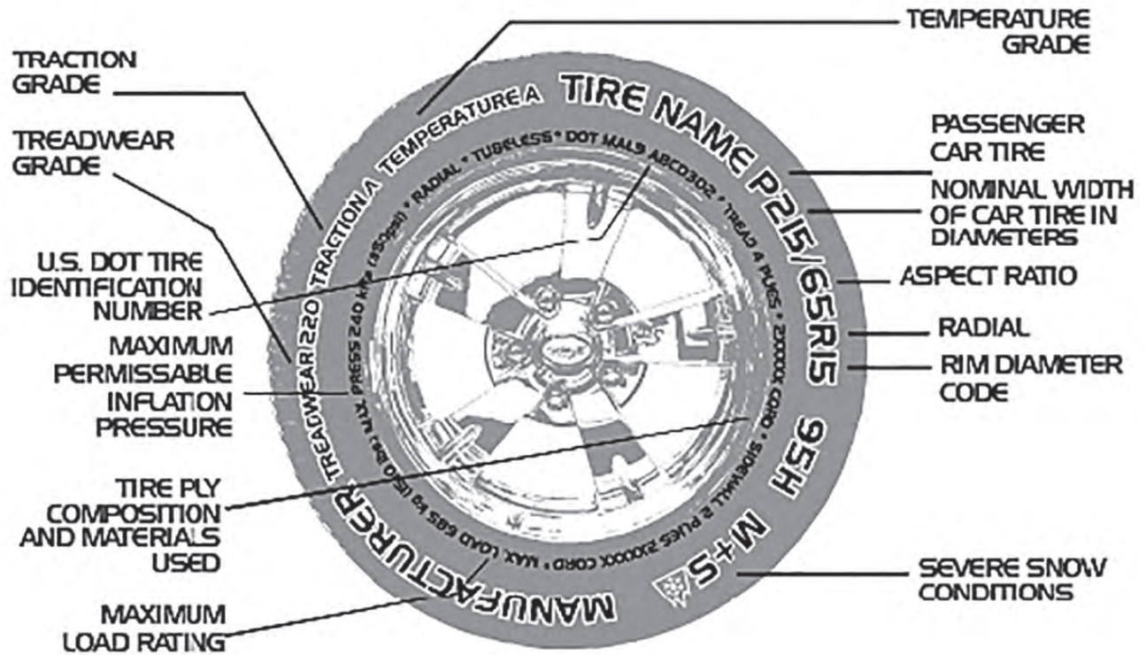
Figure 16-3: Tire information
