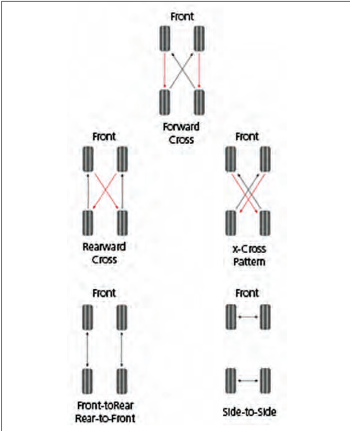
Figure 16-2: Tire rotation example
