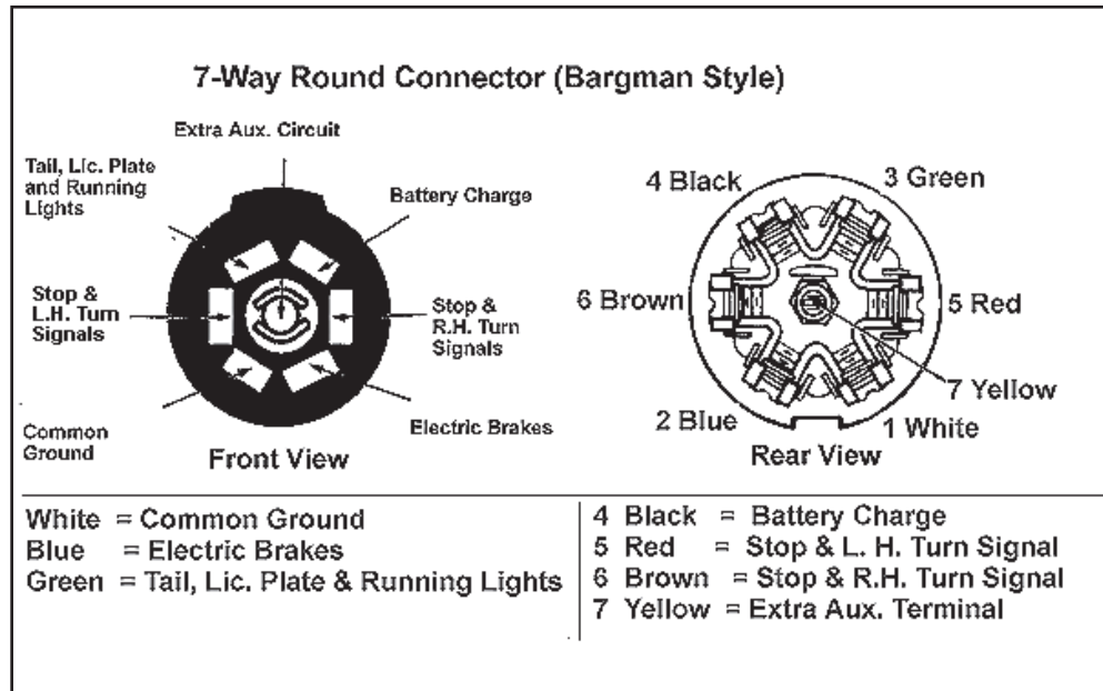
Figure 9-19: Seven-Pin towing connector
