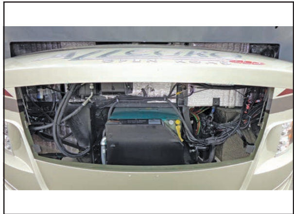
Figure 9-5: Electrical generator
