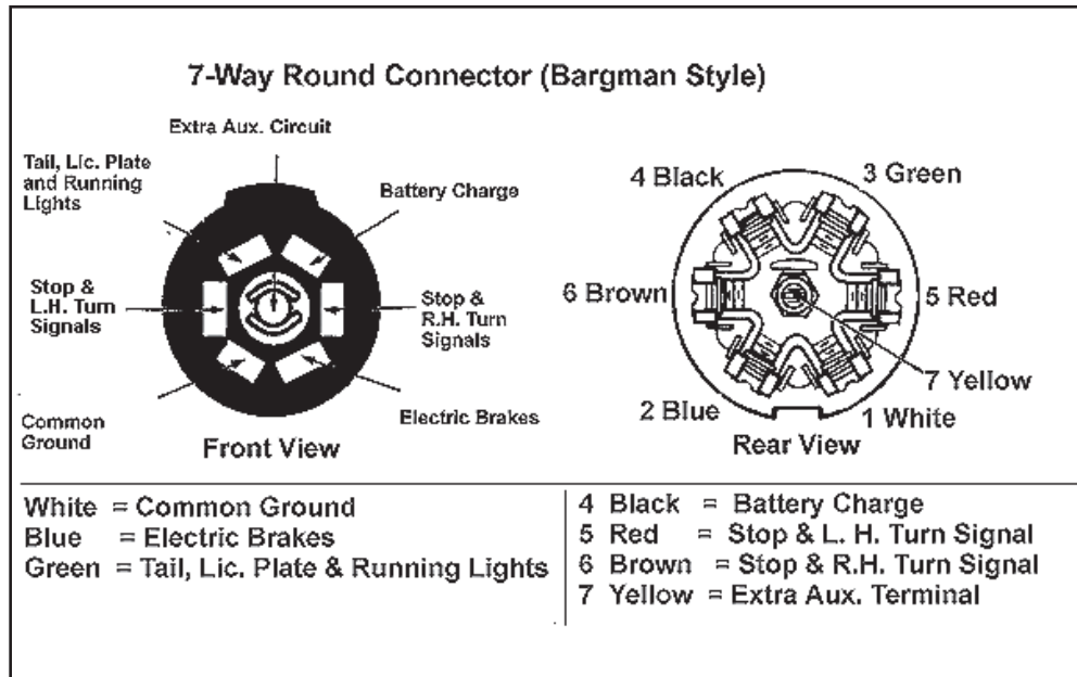
Figure 9-13: Seven-Pin towing connector
