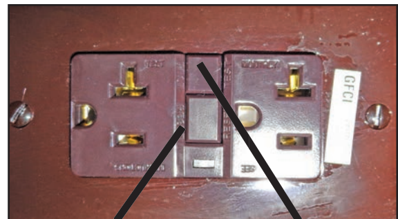
Figure 9-3: GFCI receptacle
