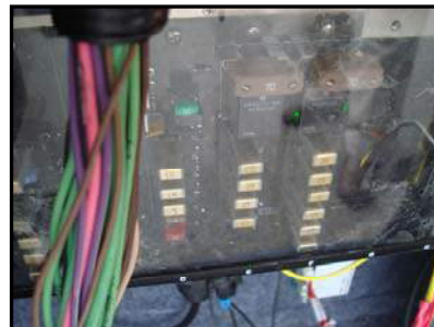
Figure 7-2. Fuse Panel
