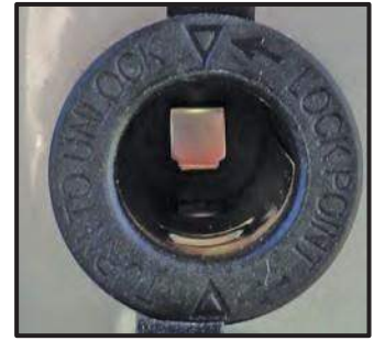
Figure 9-12: 12 VDC Receptacle
