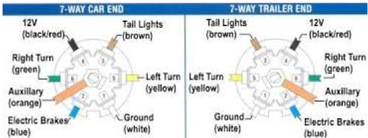
Figure 9-13: Seven Pin Connector Diagram
