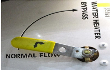
Figure 13-11: Water Heater Bypass System
