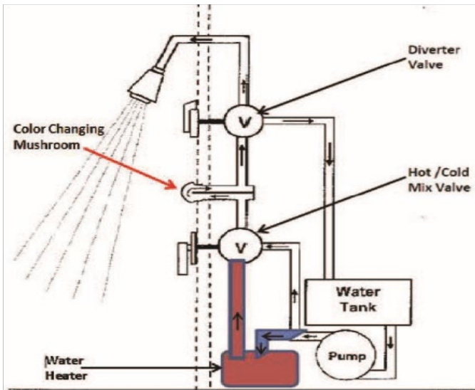
Figure 13-5: Shower Miser Diagram.
