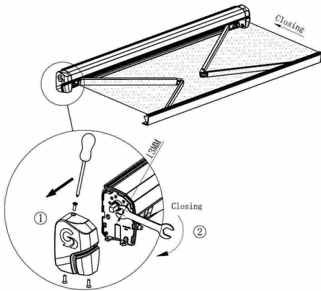
Figure 14-4: Manual Override
