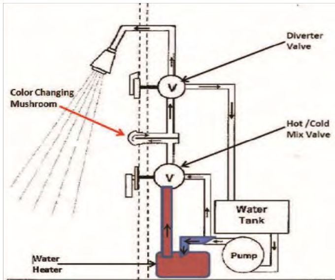
Figure 13-5: Shower Miser™ Diagram.
