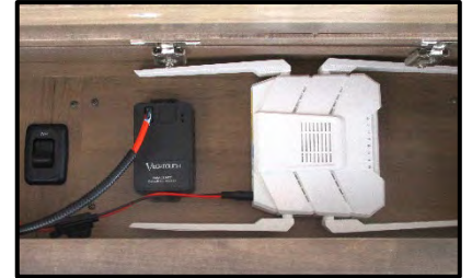
Figure 9-19 WIFI Antenna.
