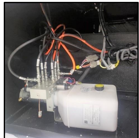
Figure 15-6a. Pump for Lippert System
