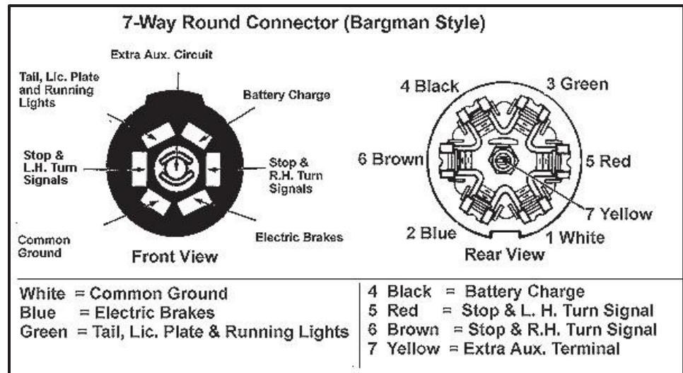
Figure 9-11: Seven-Pin Connector
