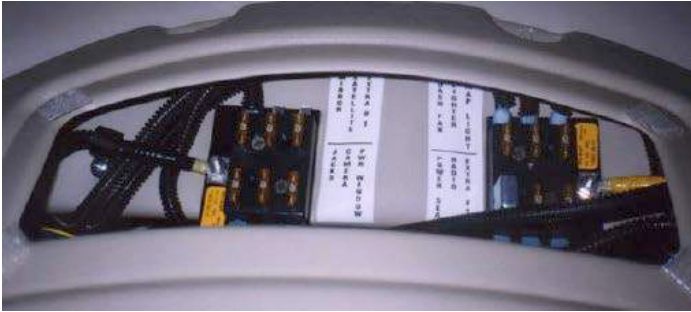
Figure 7-12. Under-dash Fuse Panels
