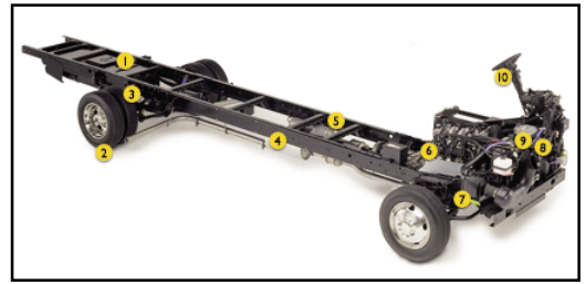
Figure 6-1. Chassis
