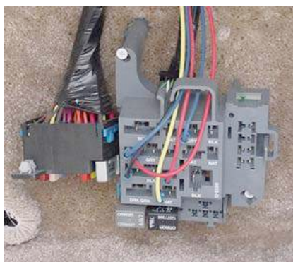
Figure 7-11. Fuse Blocks
