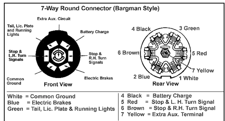
Figure 7-13. Bargman Seven-Pin Towing Connector
