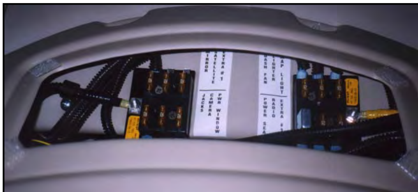
Figure 7-12. Underdash Fuse Panels
