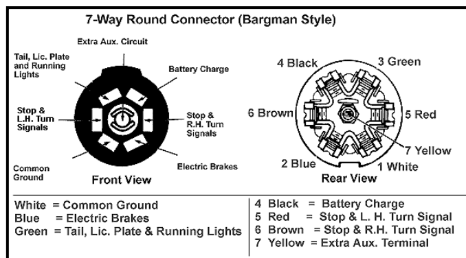
Figure 7-13. Bargman Seven-Pin Towing Connector
