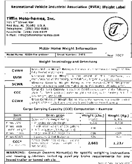
Figure 1-4. RVIA Weight Label
