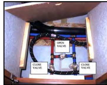
Figure 4-15. Water Heater Drain
