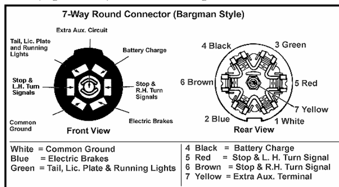
Figure 7-12. Bargman Seven-Pin Towing Connector
