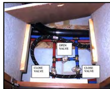
Figure 4-13. Water Heater Drain
