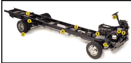
Figure 12-1. Workhorse Chassis (Typical)
