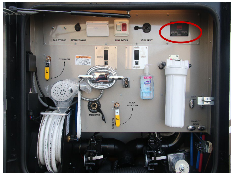
Figure 13-2: See-Level II Tank Monitor
