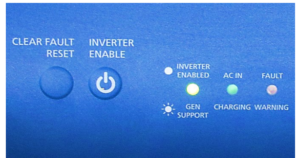
Figure 9-14: Converter/Inverter LEDs and Buttons
