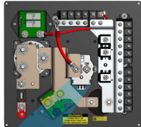
DCD Panel
