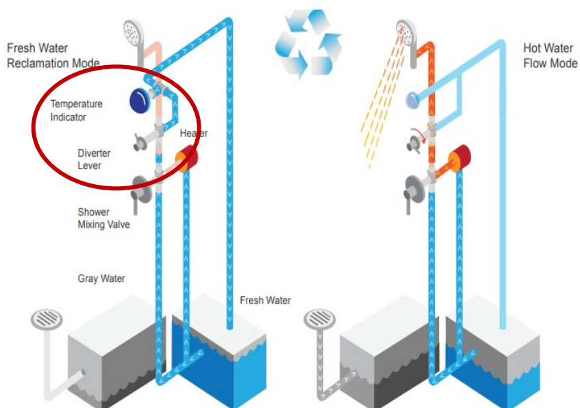
Figure 13-7: Shower Miser
