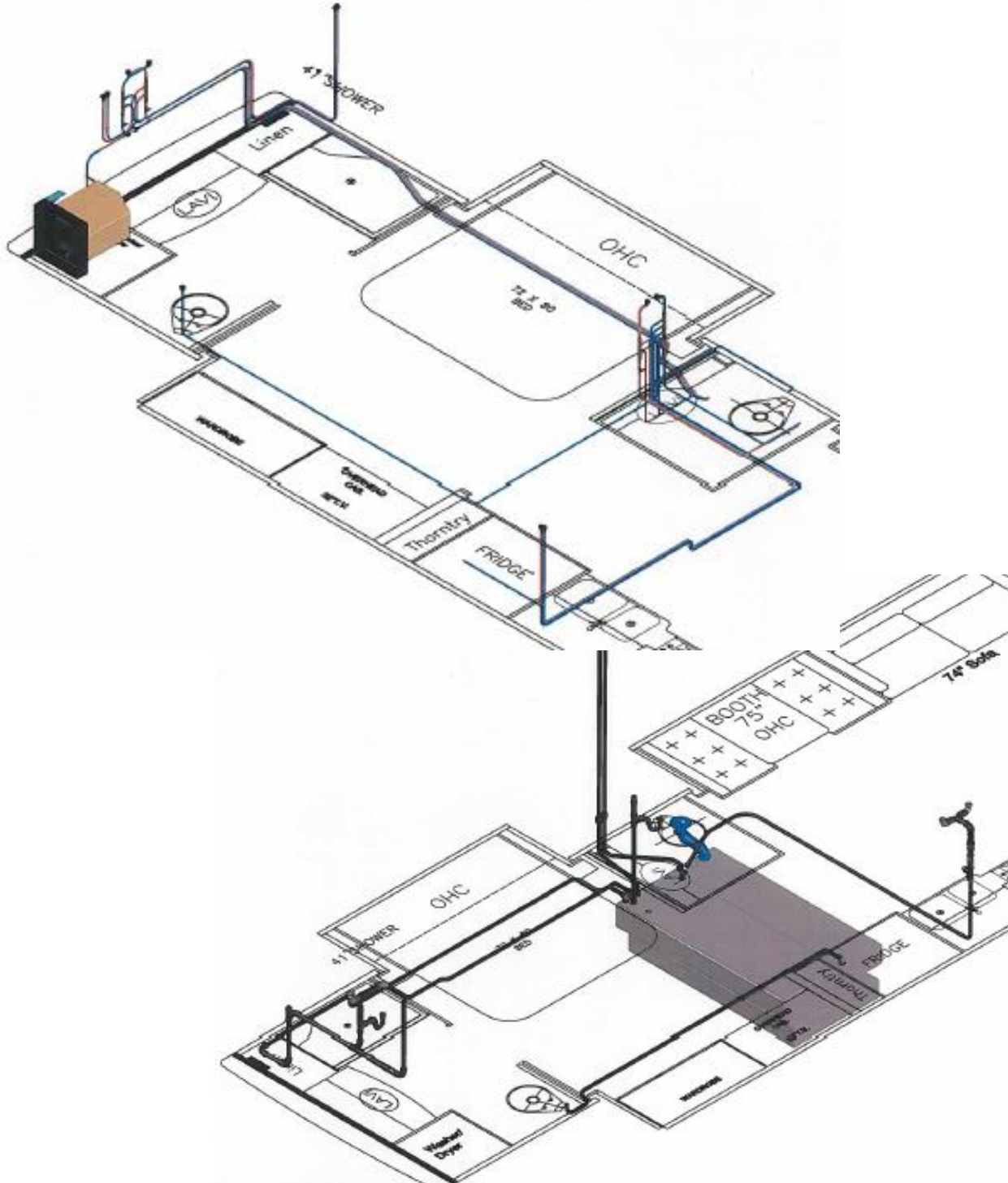
45FP Water Line Layout and Drain Line Layout
