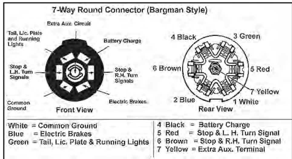
Figure 9-18: Seven-Pin Connector
