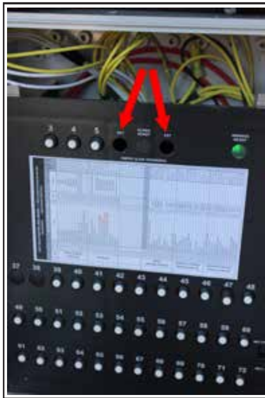
Figure 9-3 : Location of Slide-out room control override
