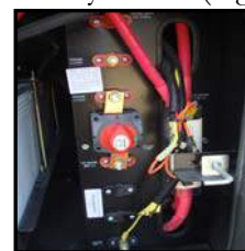
Figure 7-9. Rotary Switch to Disconnect “House” Batteries
