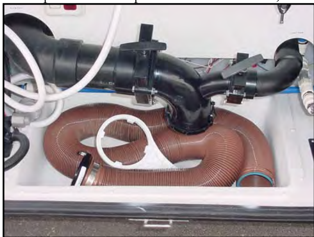
Figure 11-14. Sewer Hose and Drain Connections
