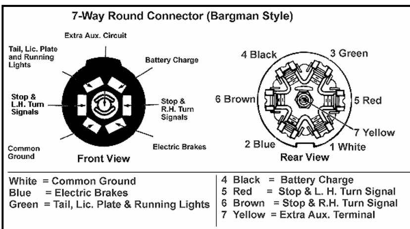
Figure 7-20. Bargman 7-Way Round Towing Connector
