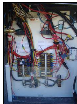
Figure 7-12. Fuse Blocks in exterior compartment on driver's side
