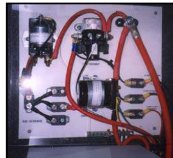
Figure 7-11. Circuit Breakers
