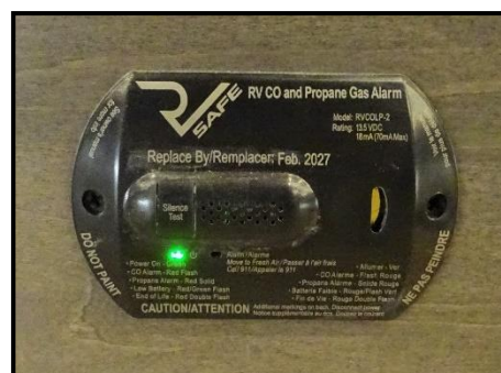
Figure 2-5: Carbon Monoxide/LP Gas Detector
